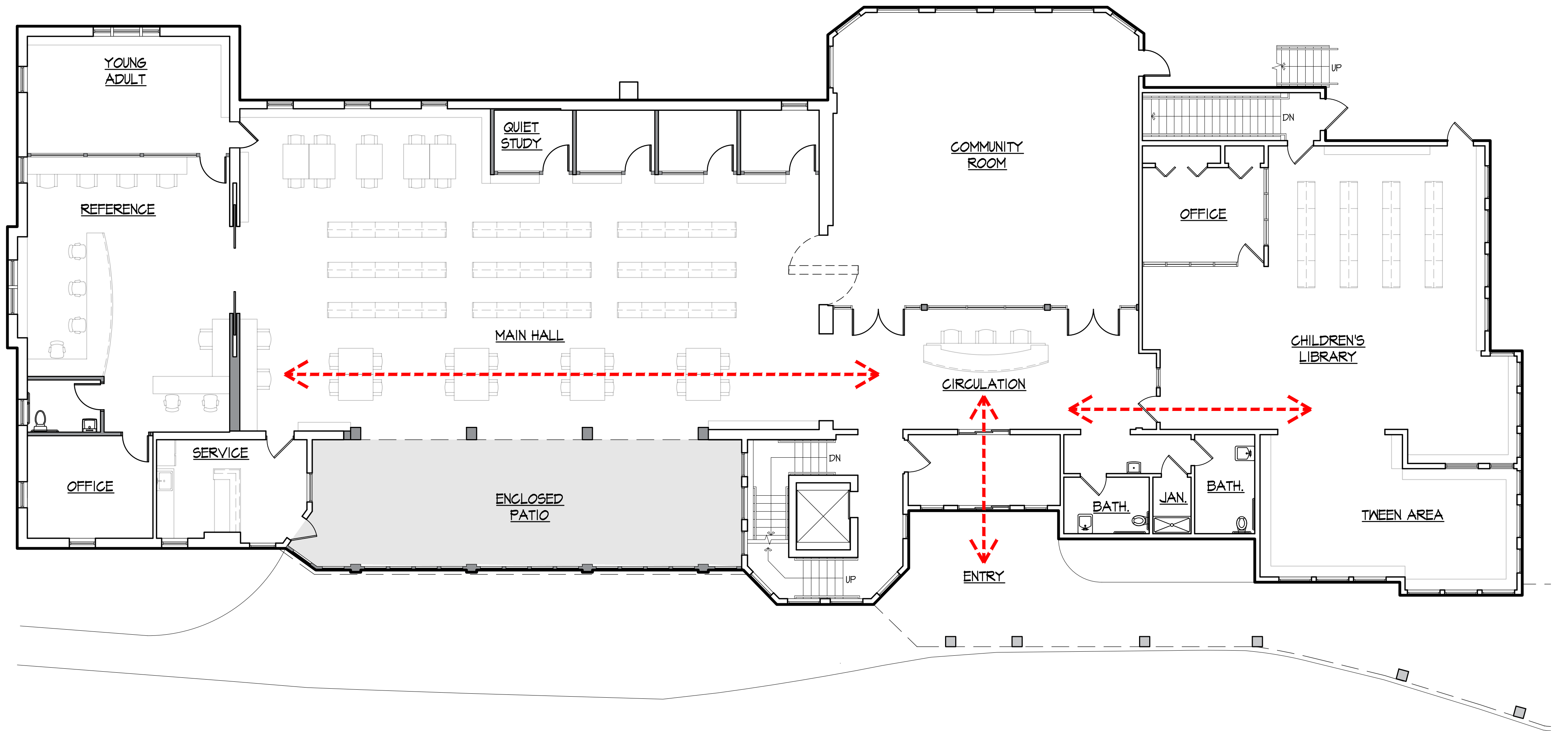
1 PROPOSED FIRST FLOOR PLAN SCALE = 1/8" = 1'-0"
